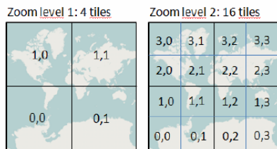
FIG 3: TILE MAP SERVICE STRUCTURE
