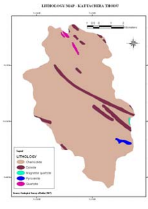
Figure 2 Rock types
